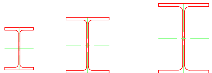
H-148x100x6x9
