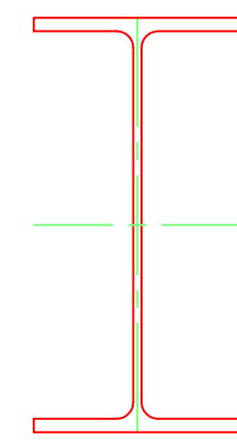
H-400x200x8x13
