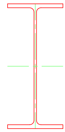
H-450x200x9x14
