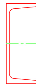
C-200x80x7.5x11
